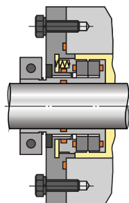
Variant 1. Springs in the medium sealed
