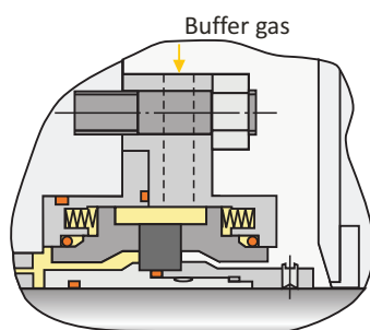
The scheme of dry gas seal for the pump
